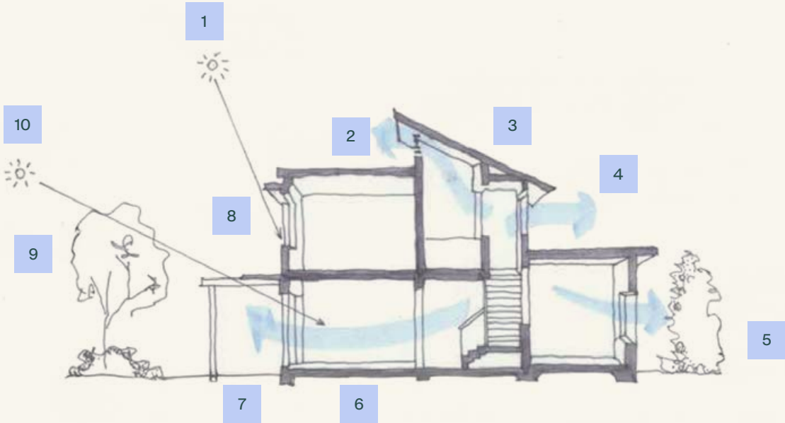
Fig 15 – Passive solar heating and cooling design
